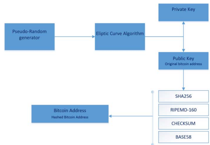
Figure 1: Bitcoin address construction
